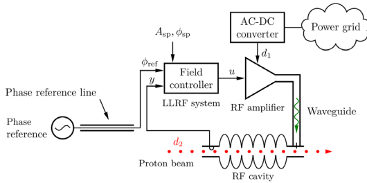
Schematic of the field-control loop at ESS.
