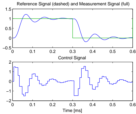
Figure 21 Control performance with interfering network messages and interfering task in the controller node.
