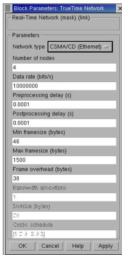
Figure 17 The dialogue of the TRUETIME Network block.
