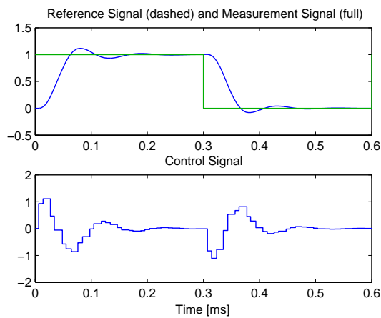
Figure 23 Control performance with delay-compensation.
